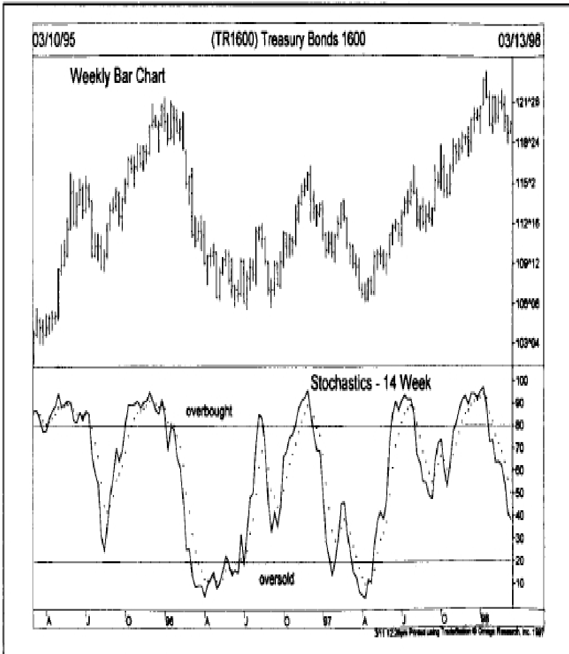
Figure 10.16 Turns in the 14 week stochastics from above 80 and below 20 did a nice job of anticipating major turns in the Treasury Bond market. Stochastics charts can be constructed for 14 days, 14 weeks, or 14 months.
