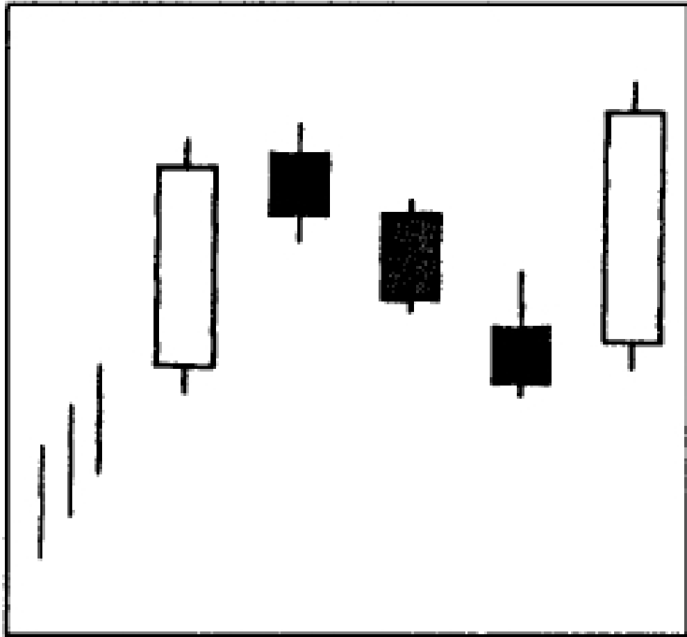
Figure 12.10 Rising Three Methods +.
