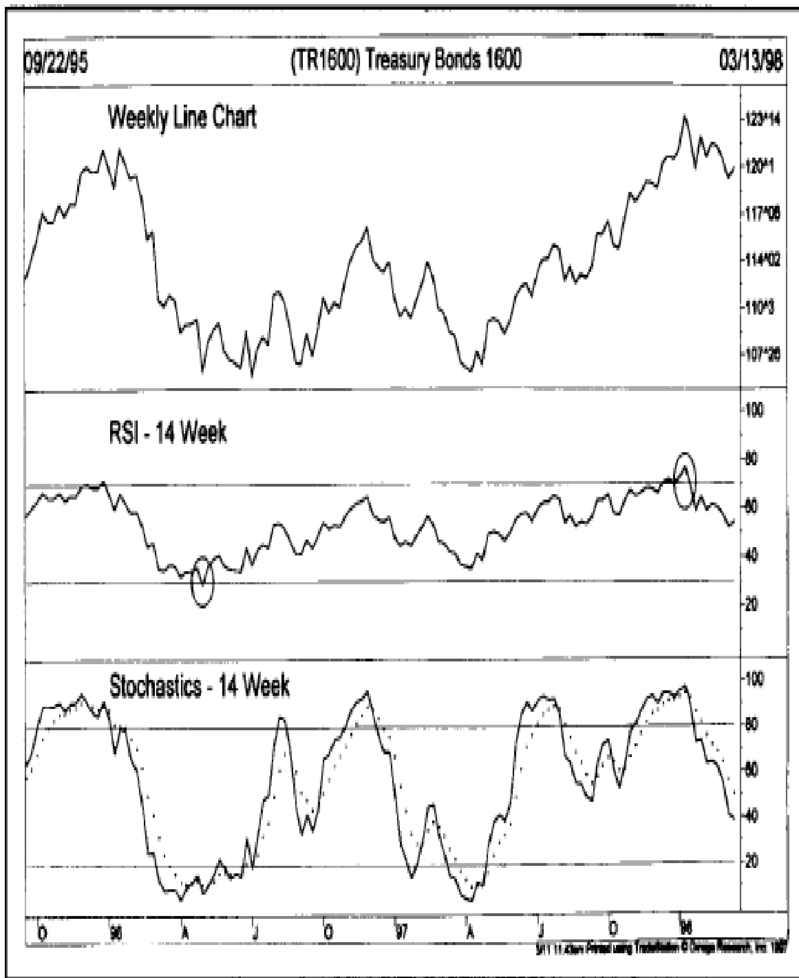
Figure 10.17 A comparison of the 14 week RSI and stochastics. The RSI line is less volatile and reaches extremes less frequently than stochastics. The best signals occur when both oscillators are in overbought or oversold territory.
