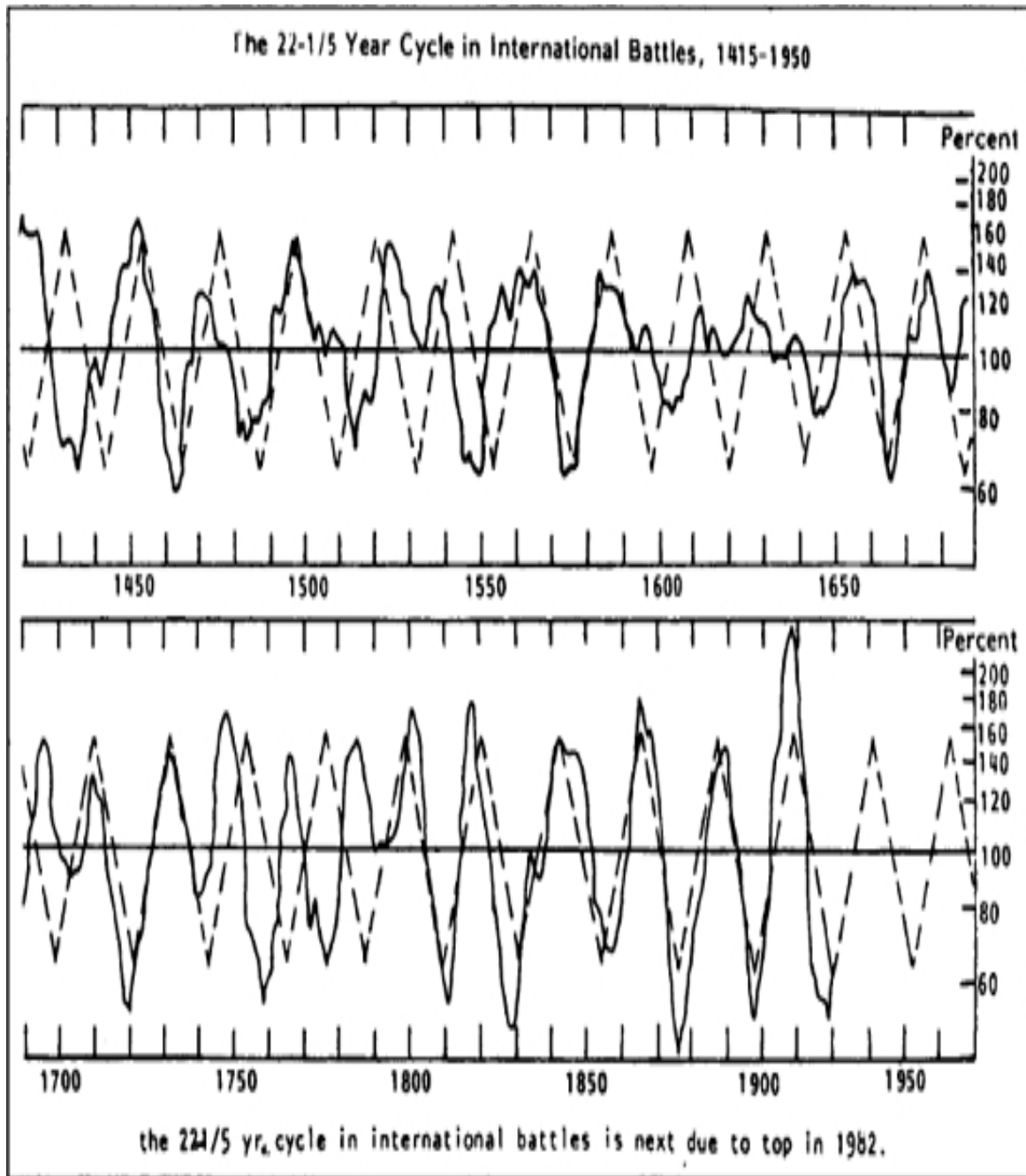
Figure 14.2 The 22.2 year cycle in international battles was due to top in 1982. In the chart, the dotted line is the “ideal” cycle, and the solid line is the actual detrended data. (Courtesy of the Foundation for the Study of Cycles, Wayne, PA.
