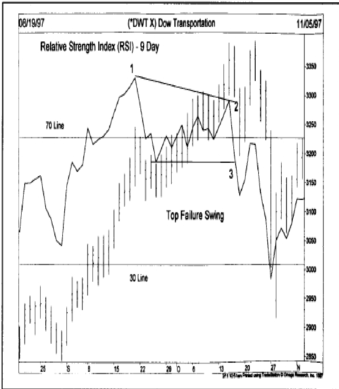
Figure 10.12b A top failure swing. The second peak (2) is lower than the first (1) while the RSI line is over 70 and prices are still rallying. The break by the RSI line below the middle trough (point 3) signals the top.
