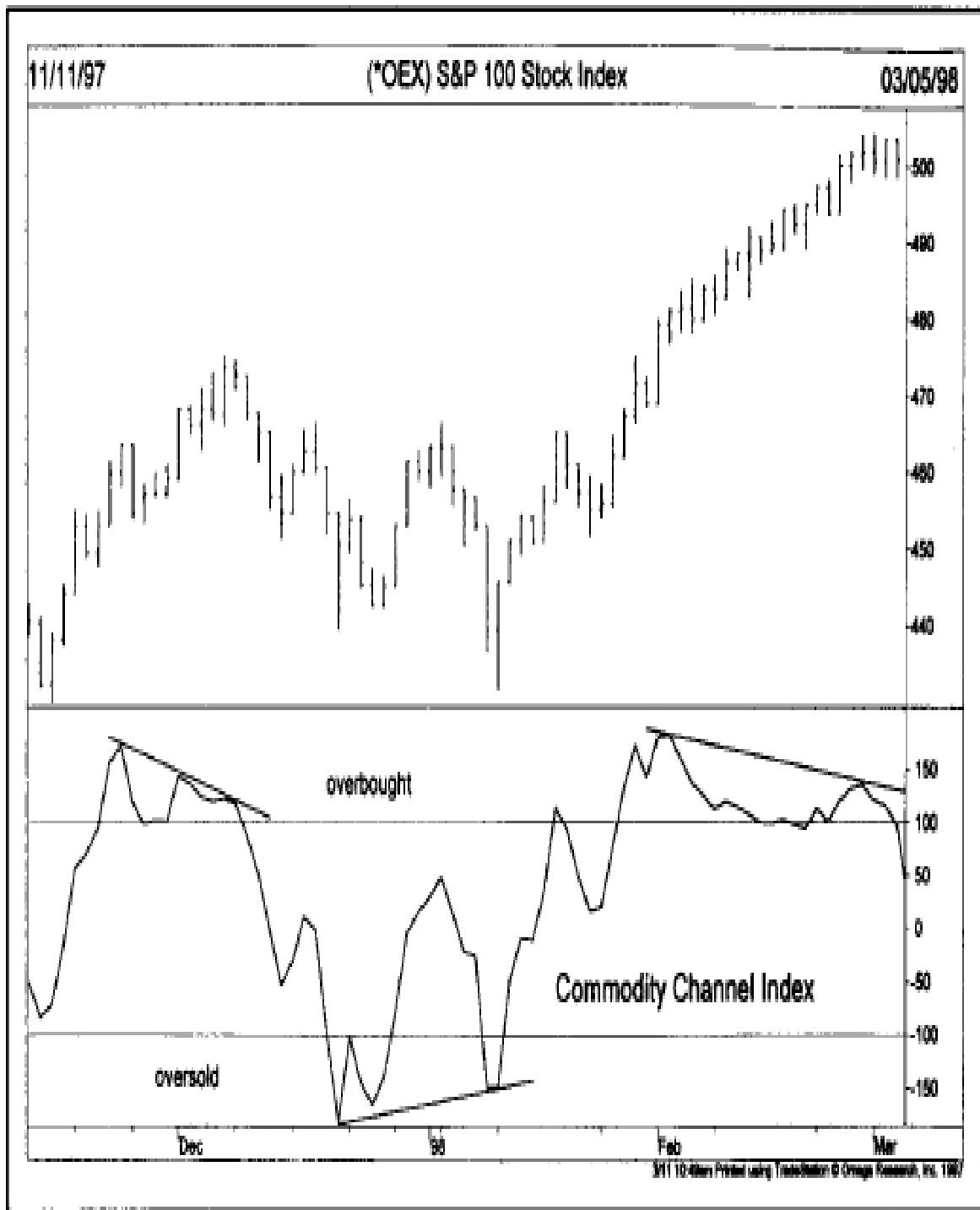
Figure 10.9 The Commodity Channel Index can be used for stock indexes like this one and can also be used like any other oscillator to measure market extremes. Notice that the CCI turns before prices at each top and bottom. The default length is 20 days.
