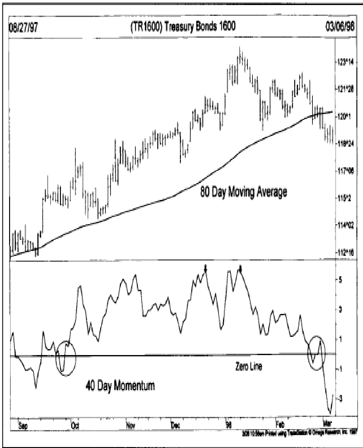
Figure 10.2b Some traders regard a crossing above the zero line as a buy signal and a crossing below the line as a sell signal (see circles). A moving average is helpful to confirm trend changes. The momentum line peaked before the price (see arrows).
